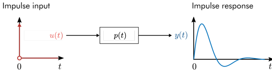
Figure 5.2: Example representation of an impulse response.
