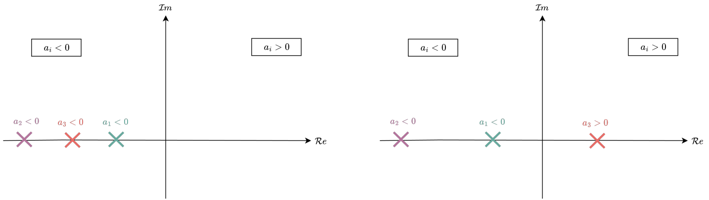
Figure 5.3: S-plane showing (left) all poles in OLHP, which implies that system response will converge to zero, and (right) one pole in ORHP, which means that system will diverge.
