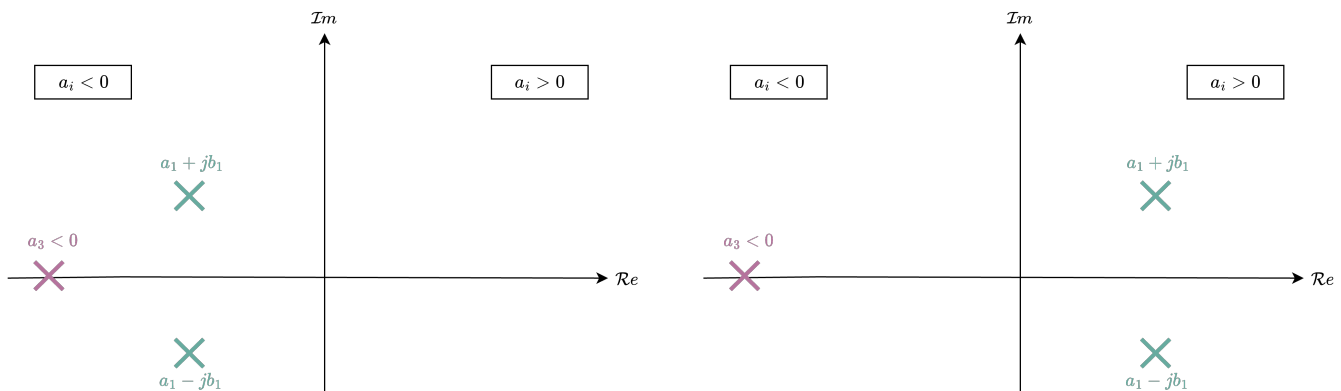
Figure 5.4: S-plane showing (left) all poles in OLHP, which implies that system response will converge to zero, and (right) one complex-conjugate pole pair in ORHP, which means that system will diverge.
