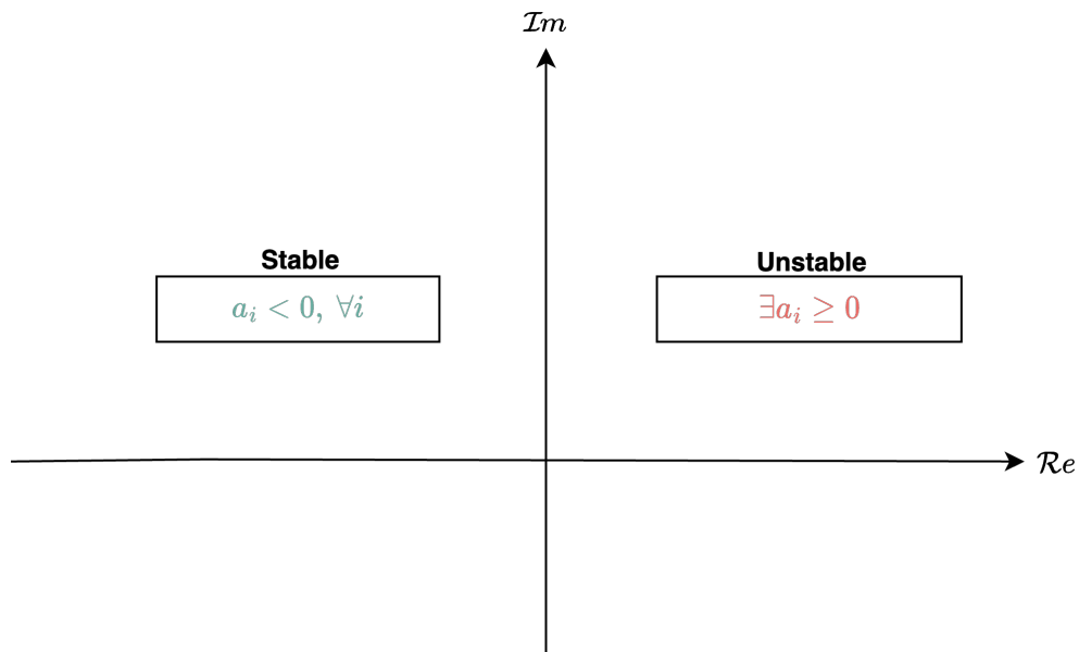
Figure 5.8: Summary of effect of pole values in s-plane on system stability.
