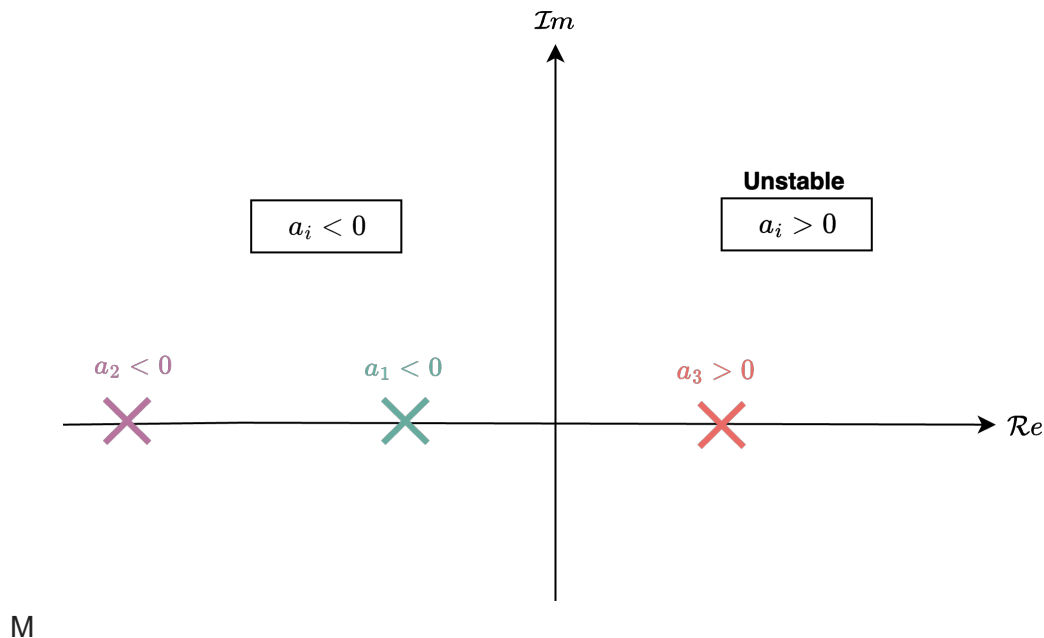
Figure 5.7: S-plane representation of an unstable system, as at least one pole is in the ORHP.
